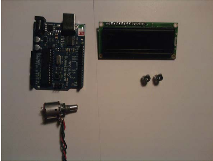
Figure 4-4. Hardware for this project (Not pictured: the USB cable, extra wire, and solderless breadboard)
